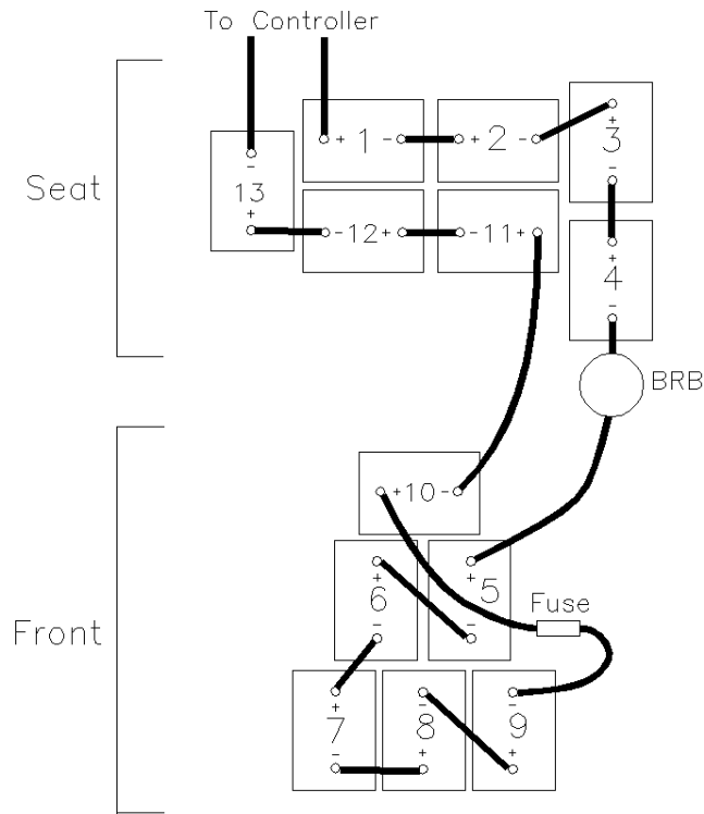
Battery map (Not to scale)
