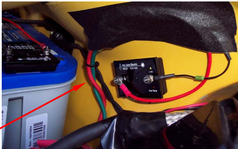
Batteries 5 and 10 installation Connect BEQ1 #5 leads to #5 battery access lead. Red lead is positive. Secure #5 wires with Gaffers tape as shown. Gaffers tape available at: http://www34.pair.com/harrison/thetapeworks.com/P009.htm
