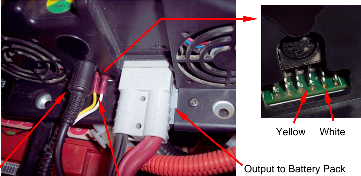
Battery Temperature Sensor
